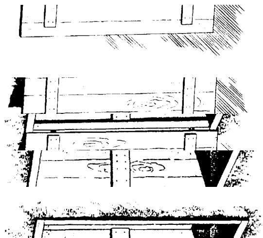
Figure 11-4.—Underground food box.
