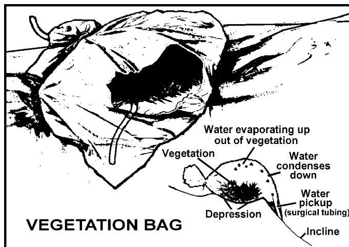
Figure VII-8. Vegetation Bag
