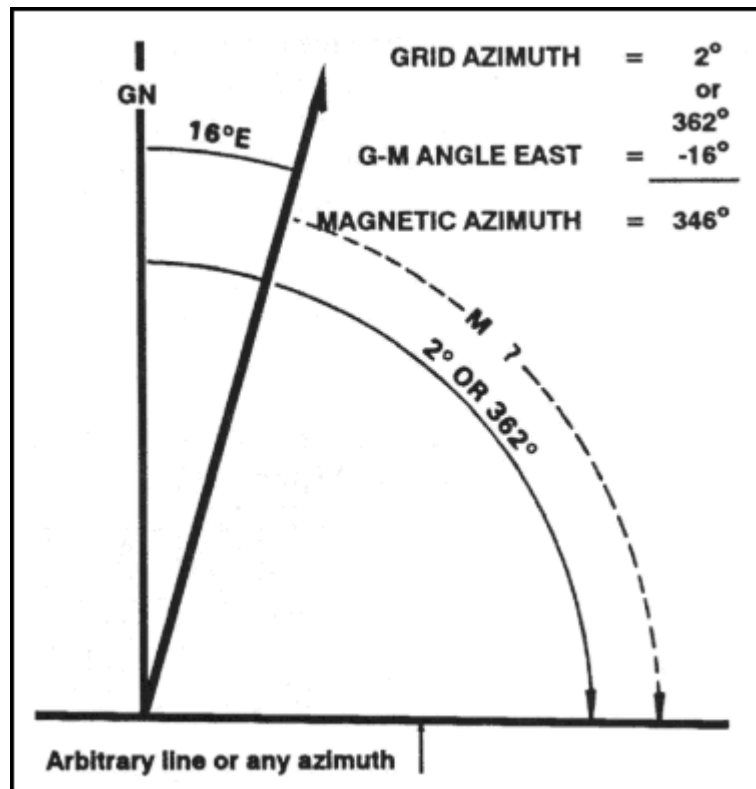
Figure 6-12. Converting to a magnetic azimuth when the G-M angle is grid.
