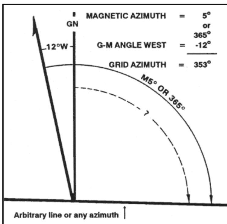
Figure 6-15. Converting to a grid azimuth when the G-M angle is greater than the magnetic azimuth.
