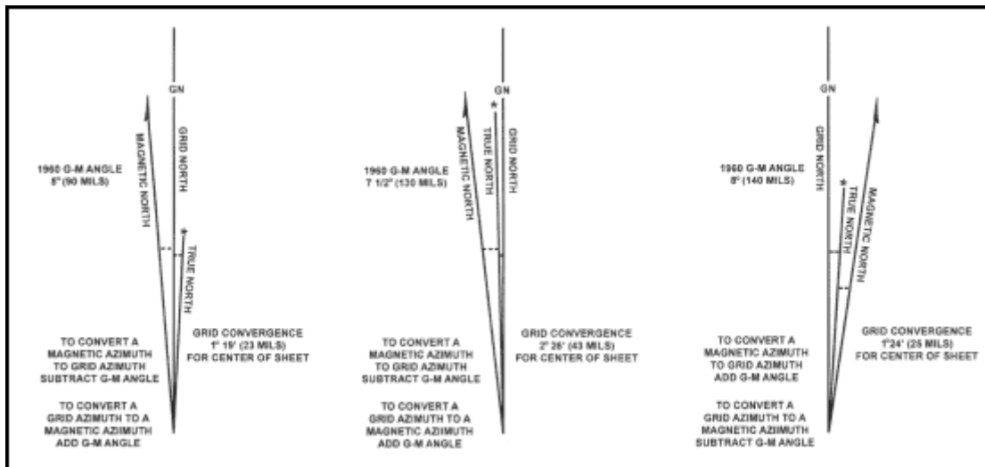
Figure 6-8. Declination diagrams.
