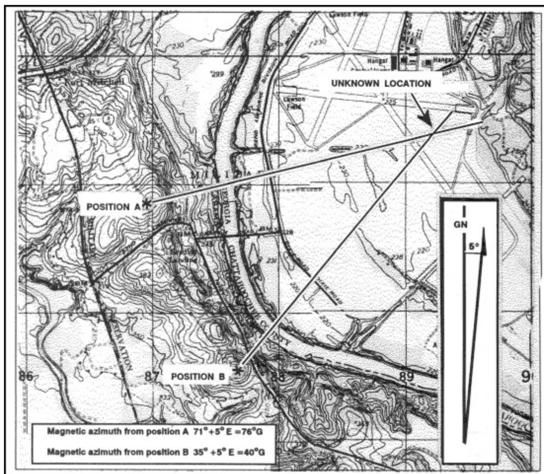
Figure 6-16. Intersection, using map and compass.
