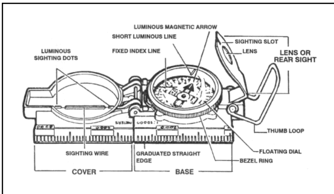
Figure 9-1. Lensatic compass.
