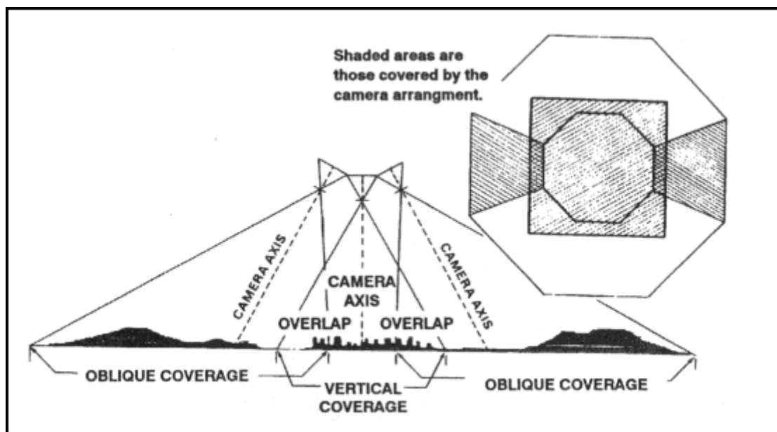
Figure 8-7. Relationship of cameras to ground for trimetrogon photography (the
