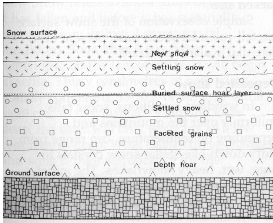
EXAMPLE SNOWPACK
