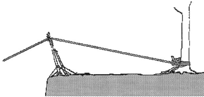
SECURING THE A-FRAME
