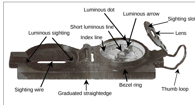
Figure 14. The Lensatic Compass
