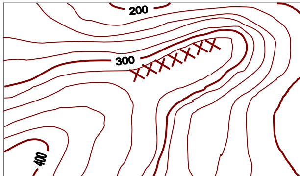
Figure 30. Ridge
