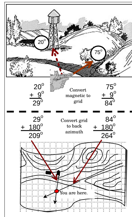
Figure 22. Calculating Azimuths
