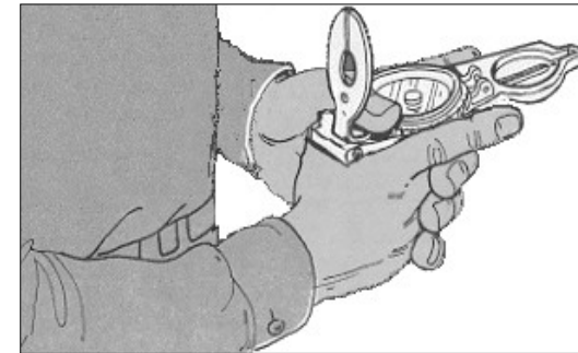
Figure 13. Center-Hold Technique
