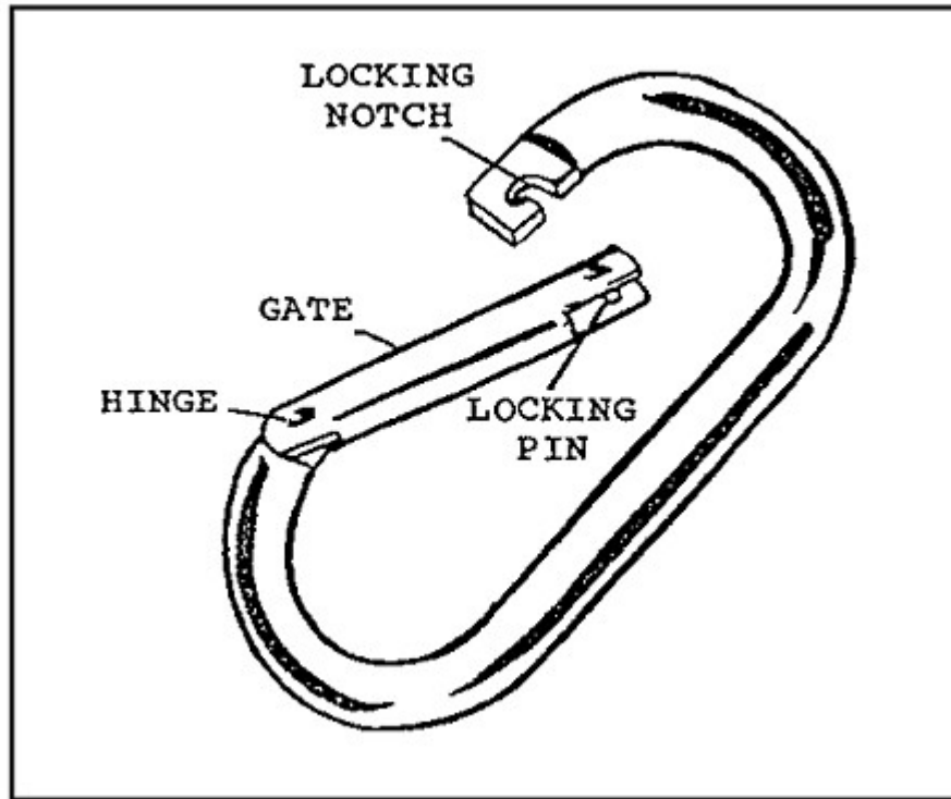
FIGURE 2-34. Snaplink (oval).
