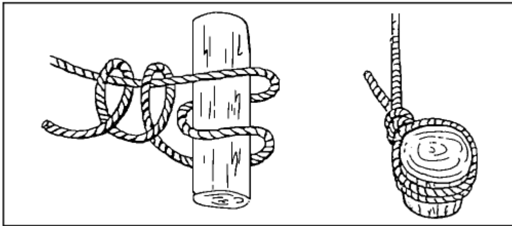
FIGURE 2-10. Double Fisherman's Knot.
